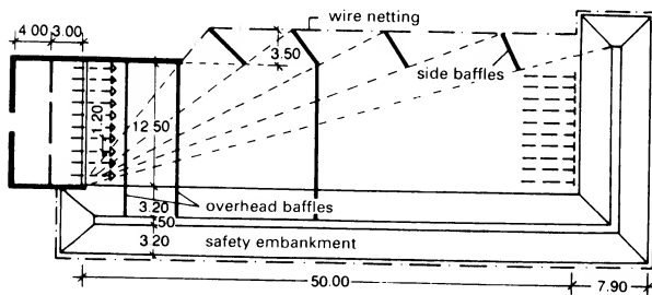
3 Small calibre range with target pulleys
